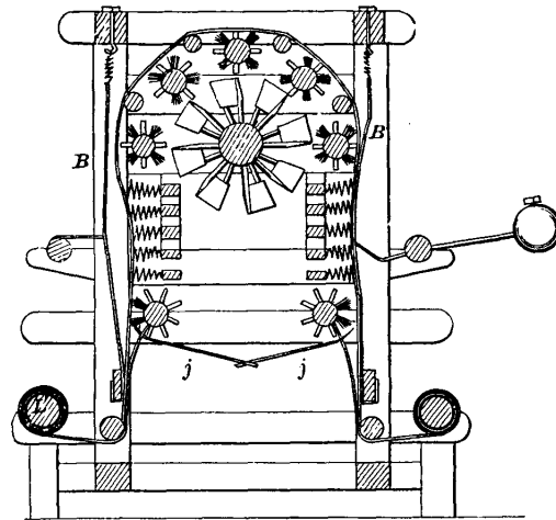
Carpet-Cleaning Machine
