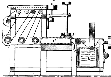
Cloth-Varnishing Machine.
