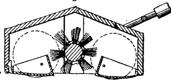
Carpet-Sweeper.
