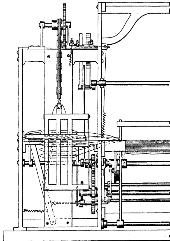
Ingrain-Carpet Loom.
