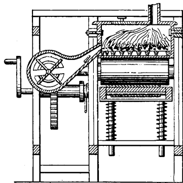
Ironing-Machine.
