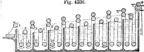
Rinsing-Machine.
