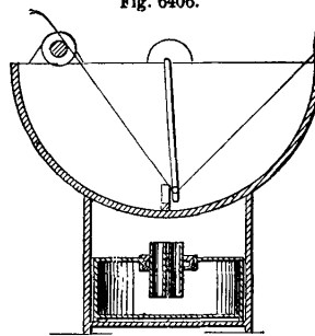
Thread-Waxer for Sewing-Machines.
