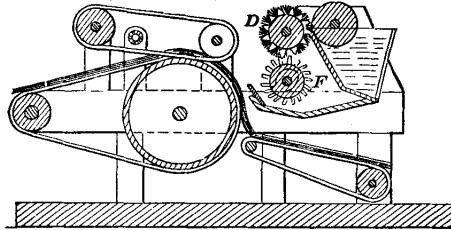
Machine for Sizing Wadding.
