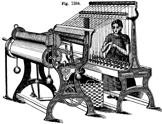
Yarn-Spooler.
