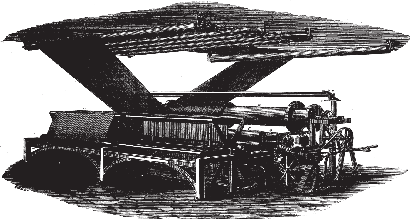
WARP-DRESSING MACHINE, CONSTRUCTED BY THE ERSTE BRÜNNER MASCHINEN-FABRIKS GESELLSCHAFT, BRÜNN.
