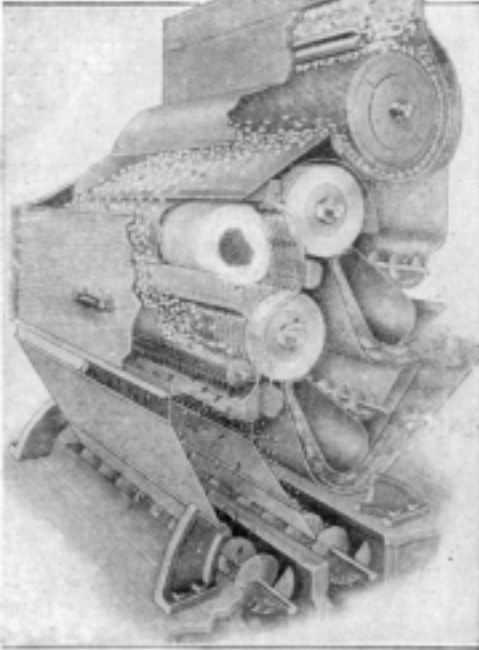
Cotton Gin with Two Sets of Saws, Which is Claimed to Give Double Capacity
