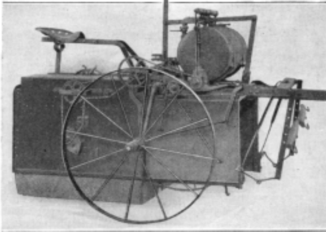
Machine for Spraying Cotton Plants with Poison, Which may Be in Either Liquid or Powder Form: The Liquid is Forced by Compressed Air through Nozzles, and the Powder Blown onto the Damp Plants
