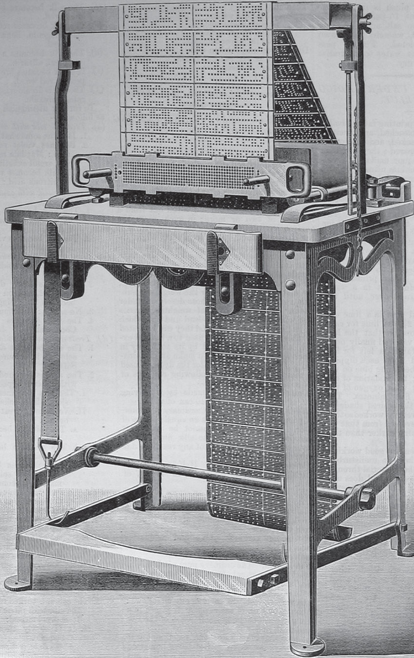
JACQUARD CARD REPEATING MACHINE TABLE.—MR. JAMES MCMURDO, MILES PLATTING, MANCHESTER.
