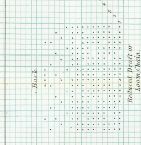
Drawing in Draft.
