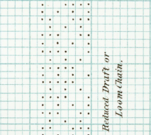
Reduced Draft or Loom Chain. Drawing in Draft.
