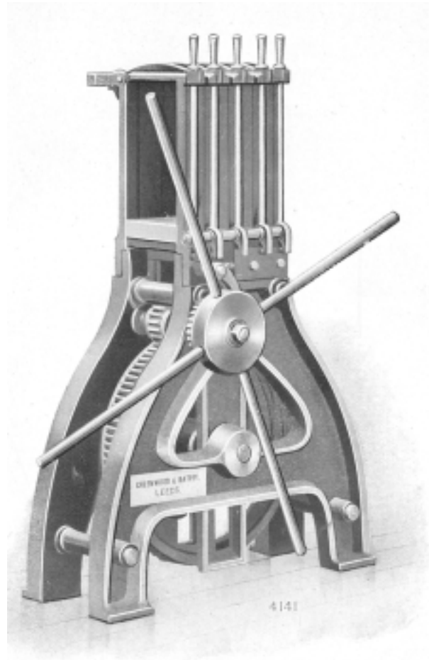
BUNDLING PRESS FOR RAMIE.
