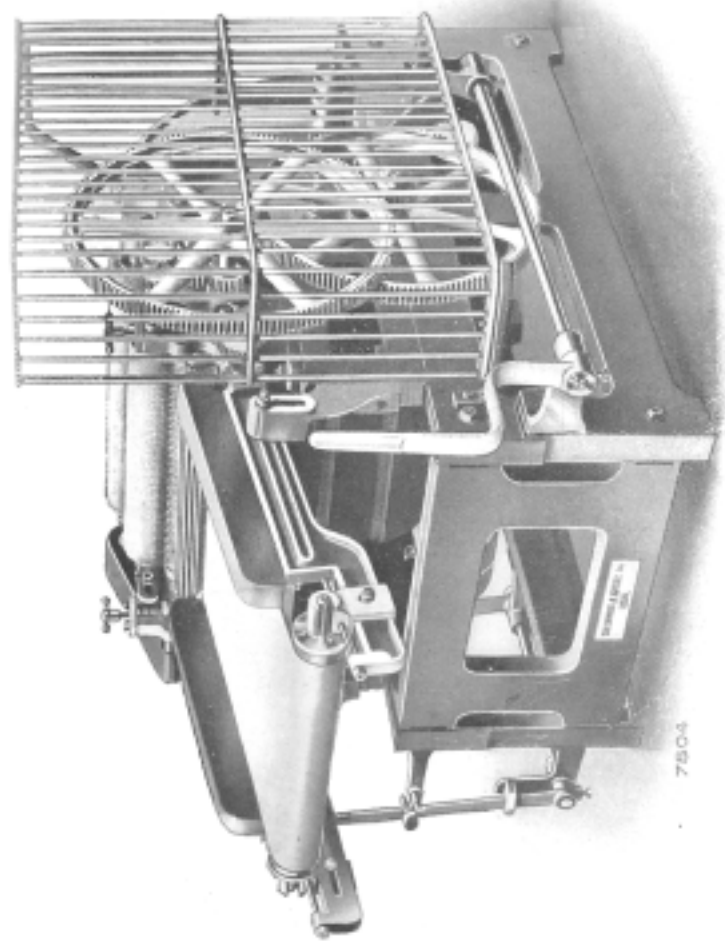
LARGE FILLING ENGINE FOR RAMIE.
