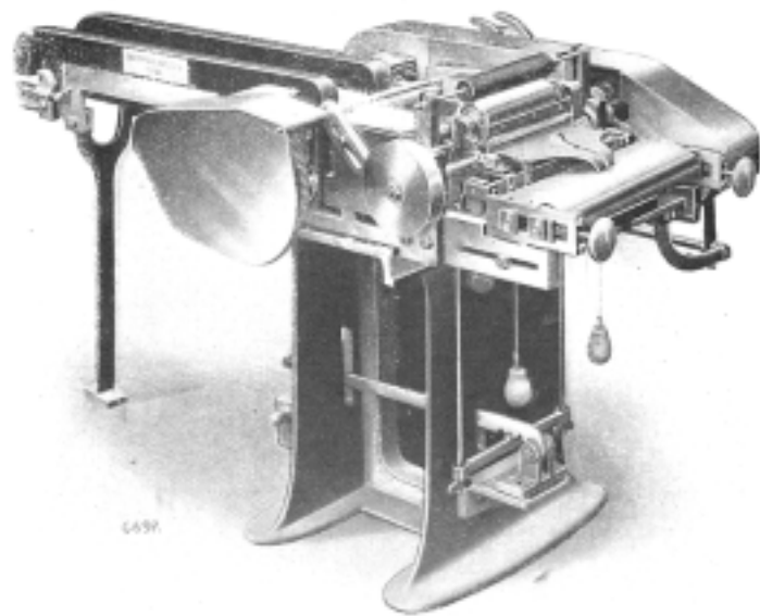
PATENT OPEN OR SINGLE SCREW GILL "SETT" FRAME FOR RAMIE.
