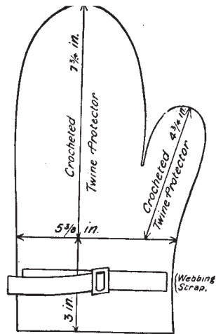
“MELLOR” MINE-SWEEPER’S GLOVE [95]
