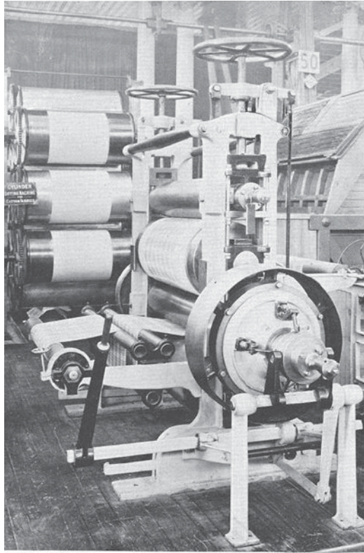
COTTON CALENDERING AND DRYING MACHINE
