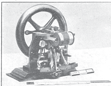
3 Howe's sewing machine, p. 61.
