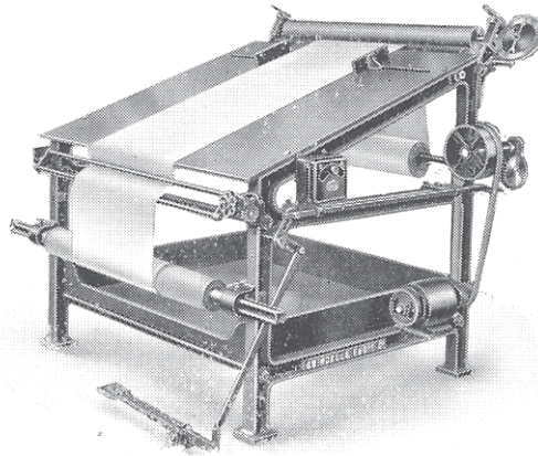
Cloth Inspecting Machine.
