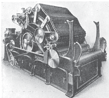
Carding Engine for Artificial Silk, Staple Fibres, "FIBRO," "Vistra," Etc.
