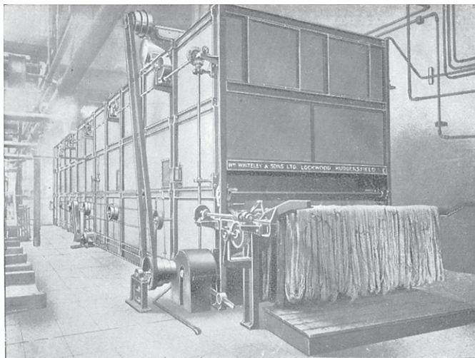
5-BAY HANK-DRYING MACHINE for Drying all kinds of HANKS
