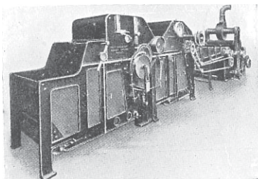
Combination of Machines for Opening and Lap Forming for Artificial Silk Staple Fibres, "Fibro," "Vistra," Etc.
