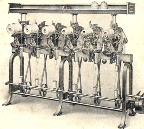
Patent "Ozri" Cone Winder winds large Cones for knitting purposes.
