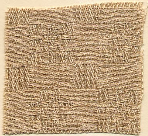
Damask diaper (40) page 31. Warp 40/2 linen at 45 ends per inch, weft 20/1. Linen from Lily Mills Company. Woven by Fred Pennington, Des Moines, Iowa.
