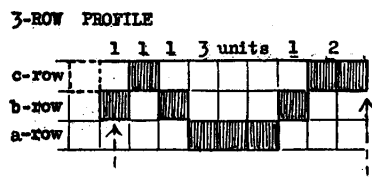
ENLARGED DRAFT OF 3-ROW PROFILE, USING 4 HARNESSES.
