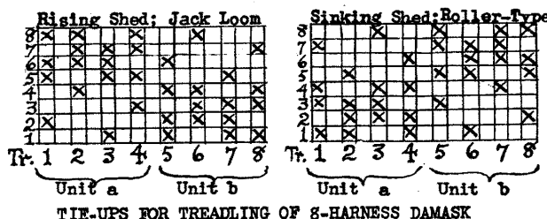
TIE-UPS FOR TREADLING OF 8-HARNESS DAMASK
