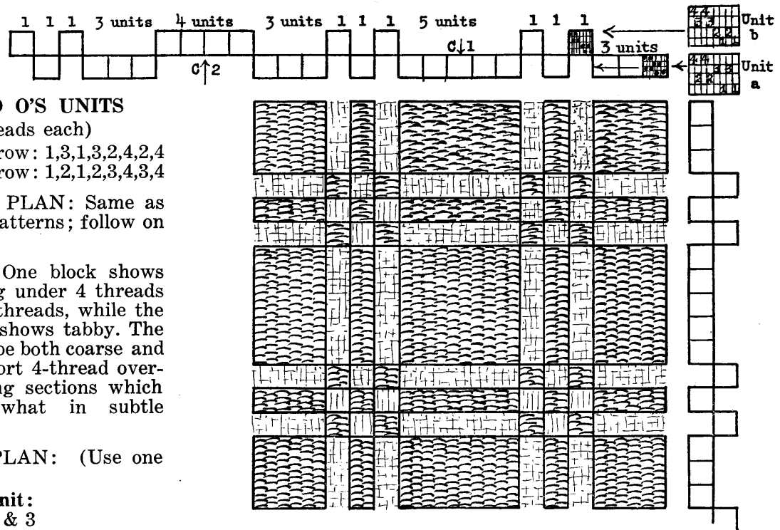
FIGURE VI—M'S and O'S PROFILE
