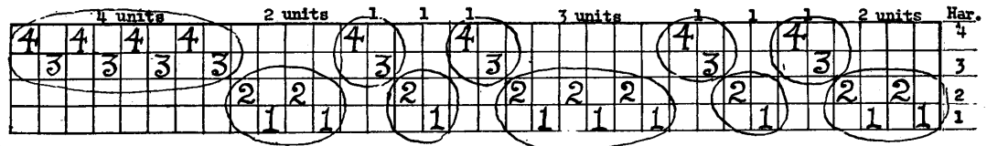
ENLARGED DRAFT OF 2-ROW PROFILE, USING 4 HARNESSES.
